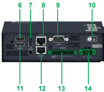
Underside view of Magelis Simple IIoT Core
